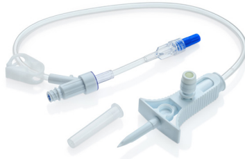
412145 Connecting Set with ULTRASITE® injection site for use with OnGuard 2 CSTD. Length: 16" (40 cm). Case Qty: 50
